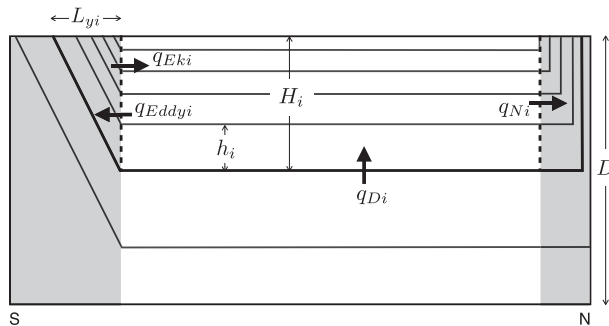
FIG. 1. Schematic of the multilayer extension of the Gnanadesikan ocean model. The model (unshaded region) represents midlatitude stratification north of the ACC, excluding the Southern Ocean and northern high-latitude basins (shaded regions).
