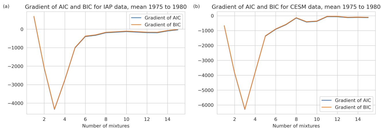
Figure 1. The AIC and BIC derivatives relative to the number of mixtures plotted against the number of mixtures. Panel a uses the IAP surface salinity distribution south of 65N over the period 1975 to 1980, while panel b uses the CESM ensemble mean surface salinity distribution over the same region and time period. The plots of AIC and BIC versus number of mixtures are in the supplement (Fig. S1).
