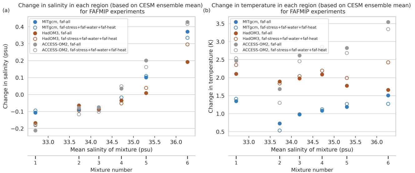
Figure 5. Comparing the surface salinity response (a) and surface temperature response (b) in each region between two cases: the sum of the response when forcings are applied individually (faf-stress+faf-water+faf-heat) and the response to all forcings applied at once (faf-all). The response is defined as the difference between the last decade of a forced run and the last decade of the control run. The response is largely linear with the exception of the sixth mixture for the HadOM3 model.
