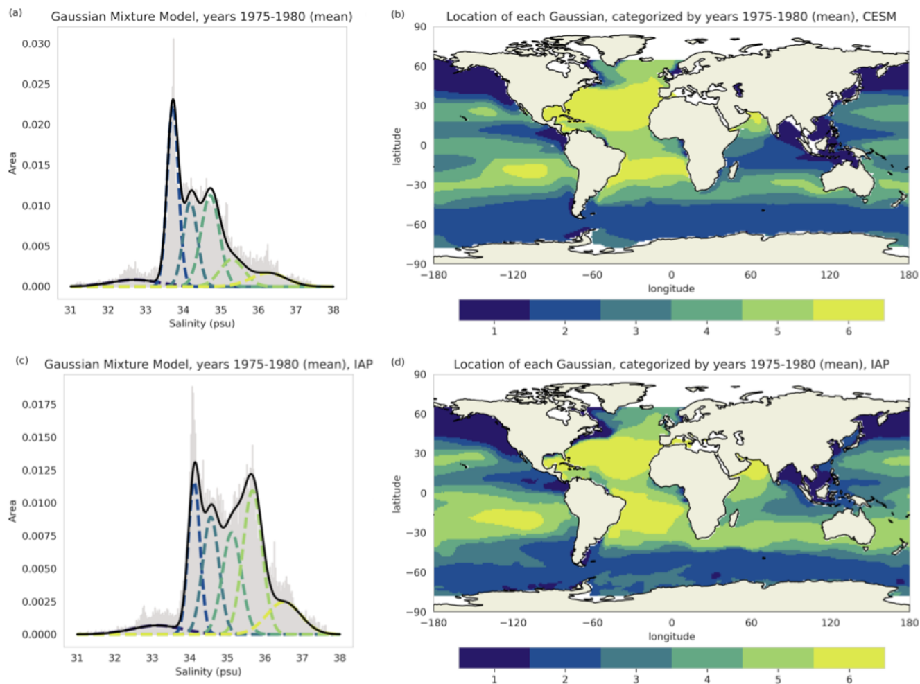
Figure 3. GMMs fit to the mean surface salinity distribution (a and c) and location of mixtures based on these models (b and d). The top row (a and b) is using surface salinity data from the CESM large ensemble with a mean across 34 members of the ensemble and over the period 1975 to 1980 (Kay et al., 2015). The bottom row (c and d) is using surface salinity data from the IAP (Cheng et al., 2020) with a mean over the period 1975 to 1980.
