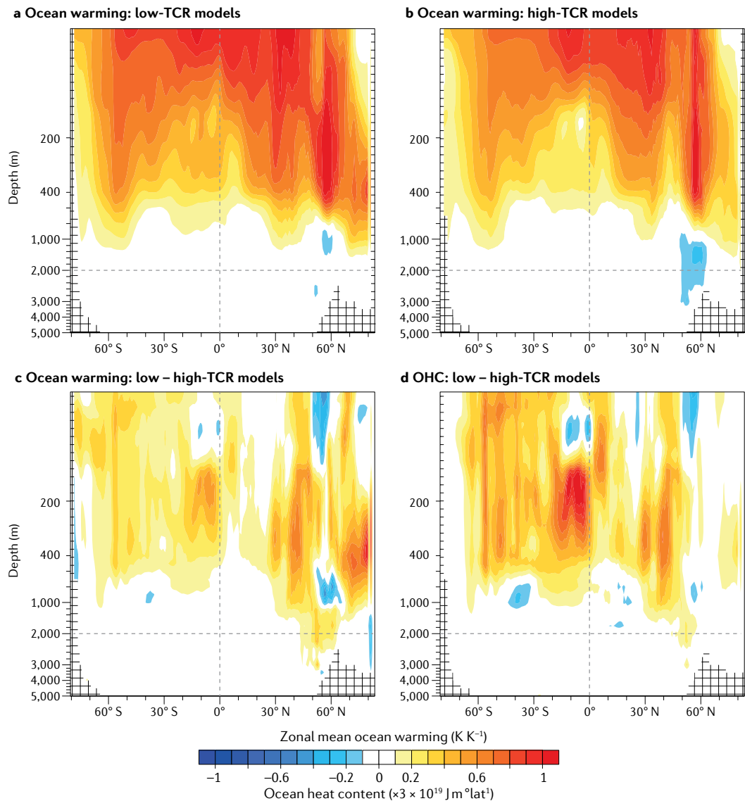
Fig. 4 | Relationship between transient climate response and the vertical structure of temperature and OHC.
